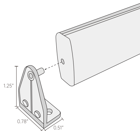
ROLLER SHADE HOLD DOWN (DETAILS)
